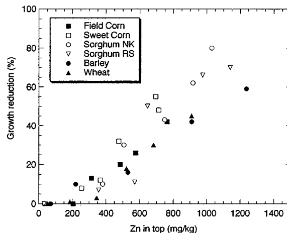
Fig. 7. Phytotoxic response to Zn in important graminaceous crops (data from Boawn and Rasmussen, 1971).
